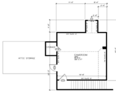
1 SECOND FLOOR PLAN SCALE 1/8"=1'-0"
